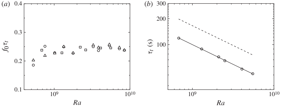
FIGURE 12. (a) Normalized switching frequency f_0 \tau_t by the LSC turnover time \tau_t as a function of Ra in the \Gamma = 1.0 horizontal cylinder. The frequency is obtained using three different methods: temperature (circles), velocity (squares) and floater (triangles). (b) Measured LSC turnover time \tau_t as a function of Ra in the \Gamma = 1.0 horizontal cylinder. The solid line is a power-law fit to the data, \tau_t = aRa^{-\gamma} , with a = 1.34 \times 10^6 and \gamma = 0.46 \pm 0.02 . The dashed line indicates the measured \tau_t in the \Gamma = 1.0 upright cylinder (Qiu & Tong 2002): \tau_t = 2.29 \times 10^6 Ra^{-0.46} .
