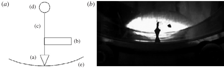
FIGURE 3. (a) Sketch of a free rotating floater used to indicate the direction of the large-scale flow: (a) cone shaped plummet, (b) rectangular flag, (c) connecting line, (d) buoyant styrofoam sphere and (e) lower conducting plate. (b) Image of an actual floater standing on the centre of the bottom conducting plate of the \Gamma = 1.69 cell. The rectangular flag points to the direction of mean flow.
