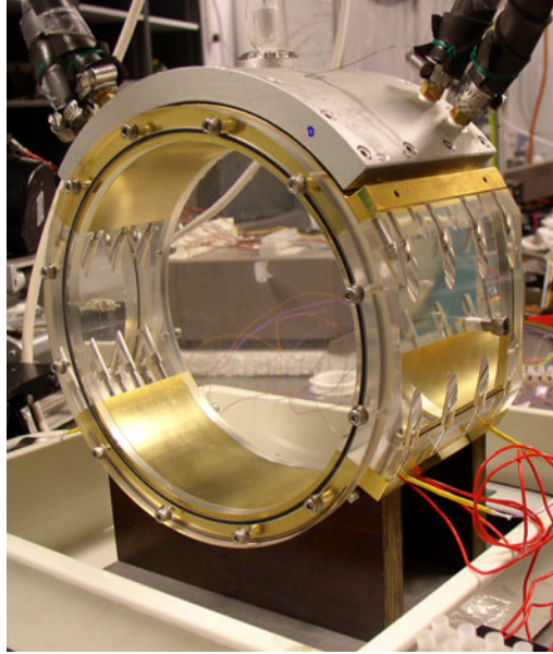
FIGURE 1. (Colour online) Assembly of a horizontal cylindrical convection cell with aspect ratio \Gamma = 0.5 . The top and bottom 1/3 of the circular sidewall of the cylinder are made of copper to provide constant cooling and heating, respectively. Sandwiched in the middle of the circular sidewall are two pieces of thermal insulating (curved) plate made of Plexiglas.
