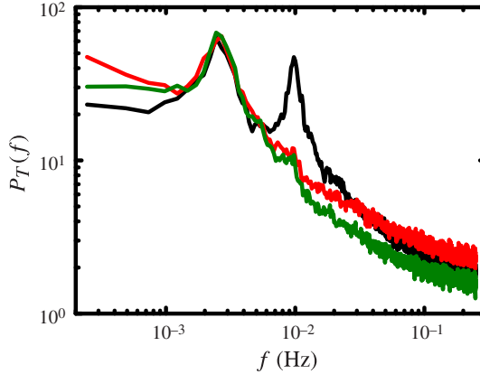
FIGURE 16. Measured power spectra P_T(f) of local temperature fluctuations at positions B (green), O (black) and C (red) as shown in figure 14.
