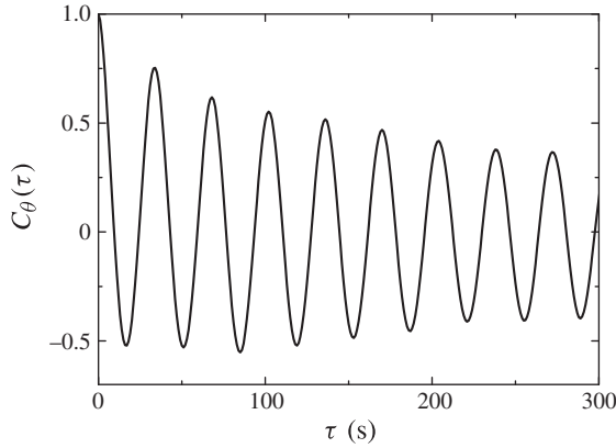
FIGURE 7. Measured auto-correlation function C_\theta(\tau) of the angular position \theta of the LSC orientation in the \Gamma = 0.7 cell at Ra = 5.5 \times 10^9 .
