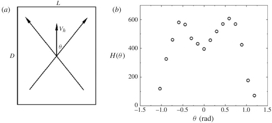
FIGURE 6. (a) Angular position \theta of the rotation plane of the LSC in the SDS phase (top view). The arrows indicate the two diagonal orientations of the LSC in the SDS phase. The rectangular box depicts the cross-sectional area at the middle height of the horizontal cylinder with L being the length of the cell and D being its diameter. (b) Measured histogram H(\theta) of the LSC orientation \theta in the \Gamma = 0.7 cell at Ra = 5.5 \times 10^9 .
