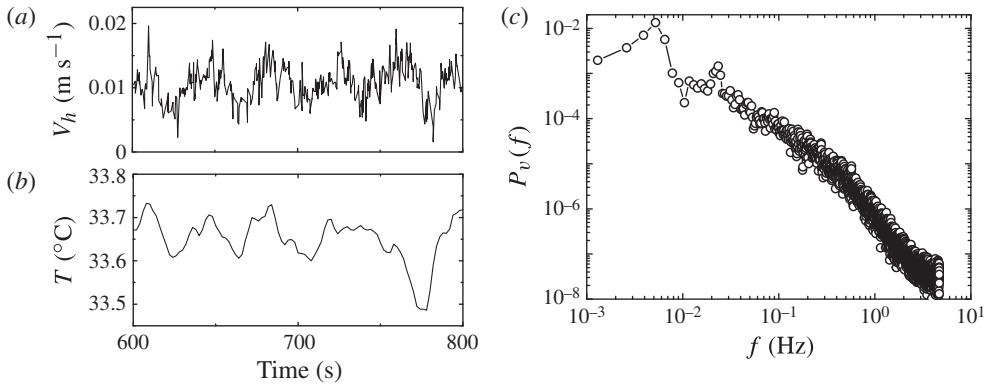
FIGURE 11. (a) Measured local velocity V_h(t) as a function of time t at 1 cm above the centre of the bottom conducting plate. (b) Time series data of the local temperature at the mid-height of the cell, 1.5 cm away from the curved sidewall. (c) Measured power spectrum P_v(f) (open circles) of V_h(t) in (a). The solid line is drawn to guide the eye. All of the measurements are made in the \Gamma = 1.0 cell at Ra = 5.5 \times 10^9 .
