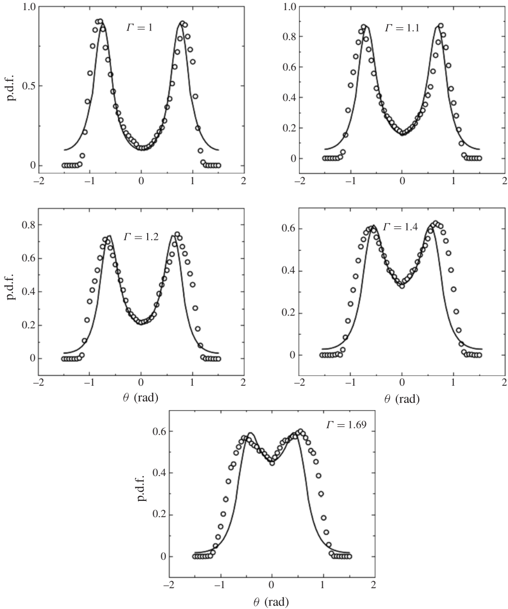
FIGURE 21. Comparison between the measured p.d.f.s P(\theta) at five values of \Gamma (open circles) and fits of the model prediction P_{\delta\alpha}(\theta) using (4.5) and (4.9) for a non-zero width LSC (solid lines). The fitting is made using \tilde{U}_0 as a free parameter. The measurements are made at Ra = 5.5 \times 10^9 and the values of \Gamma are each shown in different panels.
