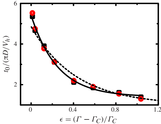
FIGURE 13. (Colour online) Normalized switching period t_0/(\pi D/V_h) as a function of the reduced aspect ratio \epsilon = (\Gamma - \Gamma_C)/\Gamma_C . The measurements are made at 1 cm above the centre of the conducting plate with Ra = 2.7 \times 10^9 (circles, shown in red online) and 5.5 \times 10^9 (black squares). The solid line is an exponential fit to the data: t_0/(\pi D/V_h) = 1.4 + 4e^{-\epsilon/\epsilon_0} , with \epsilon_0 = 0.25 . The dashed line is another exponential fit: t_0/(\pi D/V_h) = 1 + 3.86e^{-\epsilon/\epsilon_0} , with \epsilon_0 = 0.42 .
