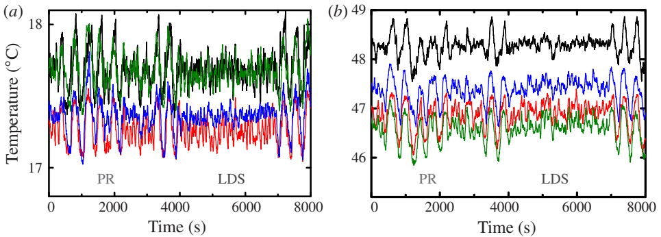
FIGURE 15. (a) Temperature signals of the top conducting plate at positions 1 (black), 2 (green), 3 (blue) and 4 (red). (b) Temperature signals of the bottom conducting plate at positions 5 (black), 6 (green), 7 (blue) and 8 (red). Measurements shown are made simultaneously with those shown in figure 14 in the \Gamma = 1.69 cell at Ra = 5.5 \times 10^9 .
