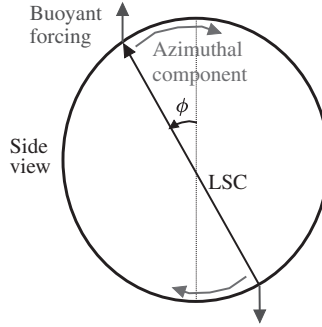
FIGURE 24. Side view of the cell illustrating the oscillation in the PR mode. The restoring force for this mode may come from the azimuthal component of a buoyant forcing on the LSC near the curved wall for \Gamma > 0.82 .
