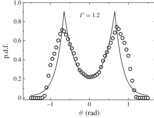
FIGURE 19. Comparison between the measured p.d.f. P(\theta) (open circles) and the calculated P_h(\theta) using (4.5) and (4.6) for a zero-width LSC (solid line). The value of \tilde{U}_0 in (4.5) is chosen to fit to the data. The measurements are made in the \Gamma = 1.2 cell at Ra = 5.5 \times 10^9 .
