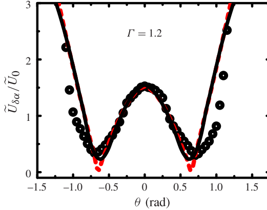
FIGURE 20. (Colour online) Comparison between the smoothed potential \tilde{U}_{\delta\alpha}/\tilde{U}_0 from (4.9) (black solid line) and the unsmoothed potential \tilde{U}_h/\tilde{U}_0 from (4.6) (dashed line, shown in red online) for the \Gamma = 1.2 cell. The two calculated potentials are normalized by a constant \tilde{U}_0 = 1/3.5 in order to compare with the measured potential \tilde{U}_m(\theta)/\tilde{U}_0 at Ra = 5.5 \times 10^9 (open circles).
