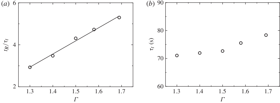
FIGURE 17. (a) Normalized rocking period t_R/\tau_t by the LSC turnover time \tau_t as a function of \Gamma at Ra = 5.5 \times 10^9 . The solid line is a linear fit, t_R/\tau_t = -5.2 + 6.2\Gamma . (b) Measured LSC turnover time \tau_t as a function of \Gamma at Ra = 5.5 \times 10^9 .
