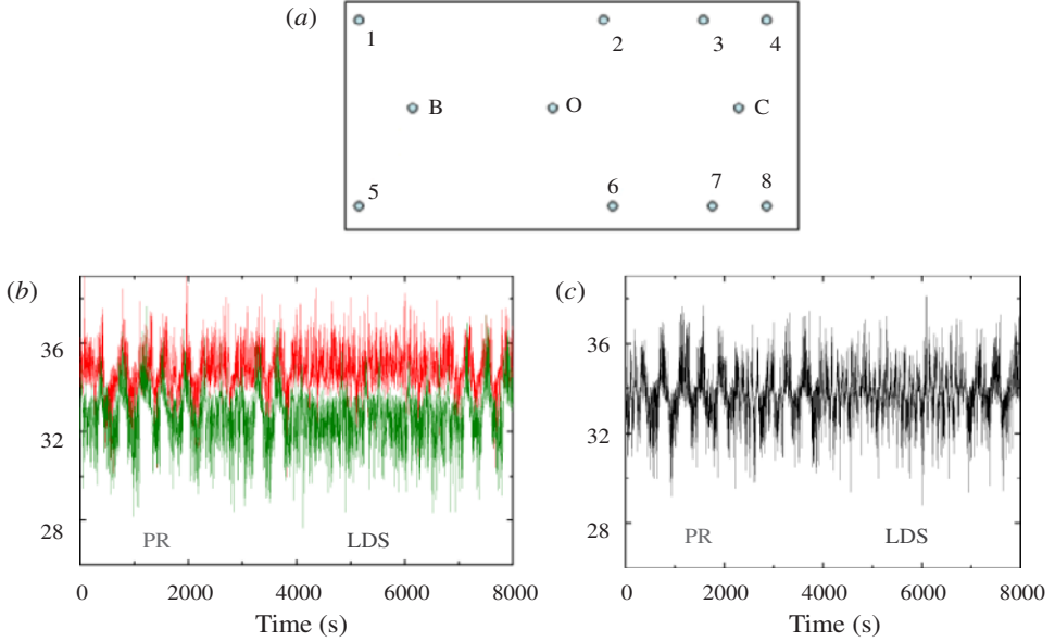
FIGURE 14. (Colour online) (a) Positions of the local temperature measurement near the curved sidewall (side view). The top and bottom four points (numbered 1–8) indicate the positions of the thermistors embedded inside the top and bottom conducting plates. The middle three points (B, O and C) indicate the positions at which the local fluid temperature is measured (15 mm away from the curved sidewall, on the same side, and at the same height). Positions B and C are D/4 (with D being the cell diameter) away from the end. Position O is 0.75D away from one side and 0.94D away from the other side. (b) Temperature signals at positions B (lower curve, shown in green online) and C (upper curve, shown in red online). (c) Temperature signal at position O. Measurements are made in the \Gamma = 1.69 cell at Ra = 5.5 \times 10^9 .
