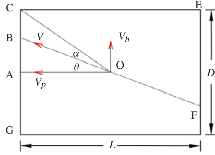
FIGURE 18. (Colour online) Top view of the horizontal cross-section of a \Gamma \geq 0.82 cell at the mid-height. Line \overline{BF} represents the instantaneous LSC orientation \theta(t) with respect to line \overline{OA} , and its length is the azimuthally varying diameter D(\alpha) with the angle \alpha being defined with respect to the diagonal line \overline{OC} . The three arrows (shown in red online) indicate the velocity coordinate system used in the LDV measurement.
