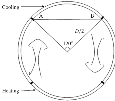
FIGURE 10. End view of the horizontal cylinder with the length \overline{AB} between the two ends of the conducting plate being (\sqrt{3}/2)D .
