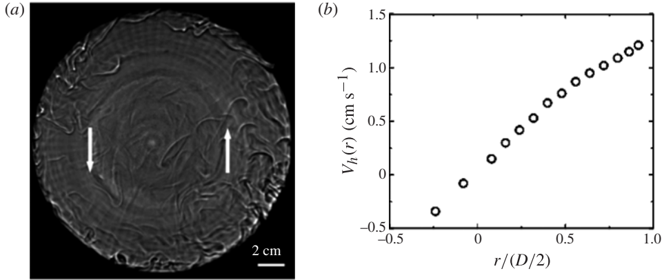
FIGURE 5. (a) A shadowgraph showing the large-scale flow and the spatial distribution of thermal plumes in the \Gamma = 0.16 cell at Ra = 4 \times 10^9 . (b) Measured horizontal velocity profile V_h(r) at Ra = 6 \times 10^9 . The measurements are made along the vertical diameter of the cell from the cell centre ( r = 0 ) to the centre of the bottom plate ( r = D/2 ).
