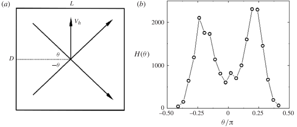
FIGURE 9. (a) Angular position \theta of the rotation plane of the LSC in the LDS phase (top view). When analysing the LDS state, we redefine the \theta = 0 position to be at the centre of the flat sidewall. The arrows indicate the two diagonal orientations of the LSC in the LDS phase. The rectangular box depicts the cross-sectional area at the middle height of the horizontal cylinder with L being the length of the cell and D being its diameter. (b) Measured histogram H(\theta) of the LSC orientation \theta in the \Gamma = 1.0 cell at Ra = 5.5 \times 10^9 . The solid line is drawn to guide the eye.
