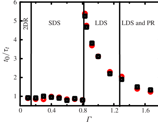
FIGURE 4. (Colour online) Normalized oscillation period t_0/\tau_t by the LSC turnover time \tau_t as a function of the aspect ratio \Gamma . The circles (shown in red online) are obtained at Ra = 2.7 \times 10^9 and the squares (shown in black) are obtained at Ra = 5.5 \times 10^9 .
