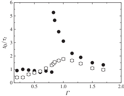
FIGURE 23. A comparison between values of the normalized period t_0/\tau_t of switching oscillations in the SDS and LDS states as a function of aspect ratio \Gamma . Solid circles: experimentally measured. Open circles: numerical solutions of the resonant frequency obtained from the Brown–Ahlers model for a rectangular cross-section with parameter values explained in the text.
