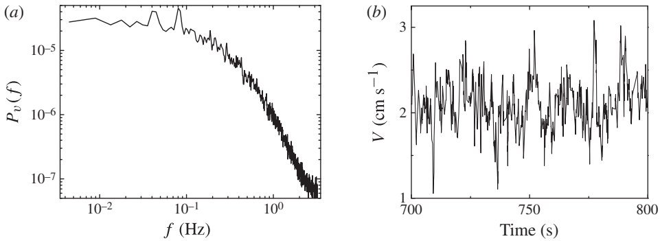
FIGURE 8. (a) Measured power spectrum P_v(f) of the horizontal velocity V_h(t) in the \Gamma = 0.5 cell at Ra = 5.5 \times 10^9 . (b) Time series data of the measured V_h(t) .
