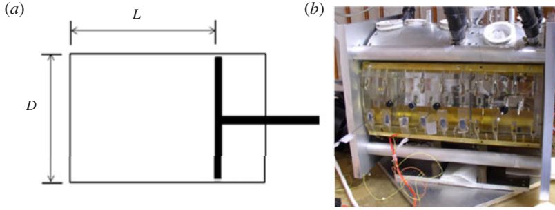
FIGURE 2. (Colour online) (a) Sketch of the \Gamma = 1.69 horizontal cylindrical cell with a mobile piston installed so that the length L of the left flow chamber can be varied in the range of 0–30 cm. (b) Assembly of the \Gamma = 1.69 horizontal cylindrical cell (without piston).
